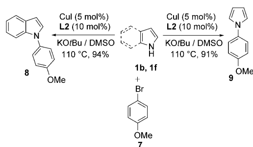
Scheme 2. Control experiment confirming N arylation
